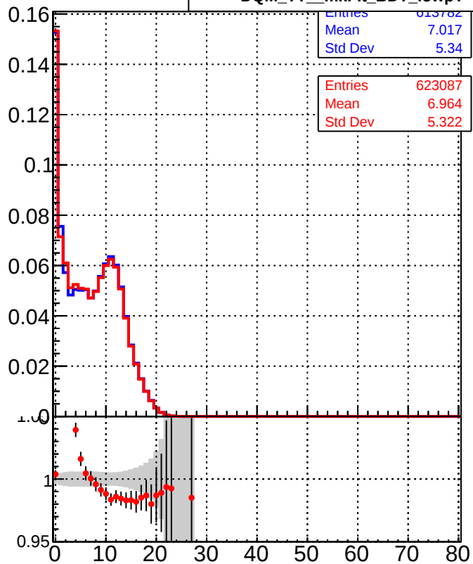
— DQM_TT_mkFit_lowpT — DQM_TT_mkFit_BDT_lowpT
