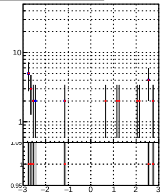
N of associated (recoToSim) tracks vs \eta Legend: DQM TT mkFit lowpT (blue dots) DQM TT mkFit BDT lowpT (red dots)
