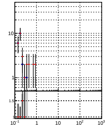
N of associated (recoToSim) tracks vs \eta Legend: DQM TT mkFit lowpT (blue dots) DQM TT mkFit BDT lowpT (red dots)
