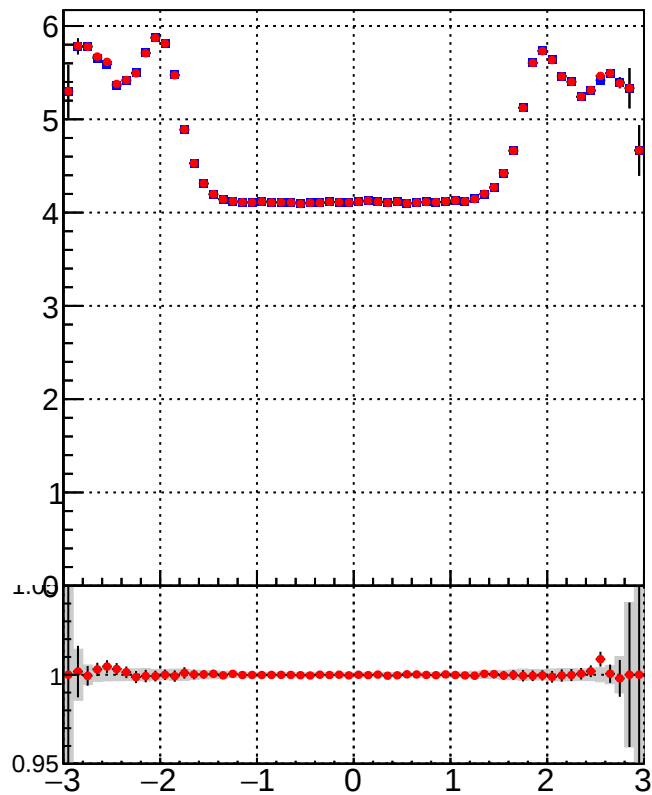
— DQM_TT_mkFit_BDT_lowpT
