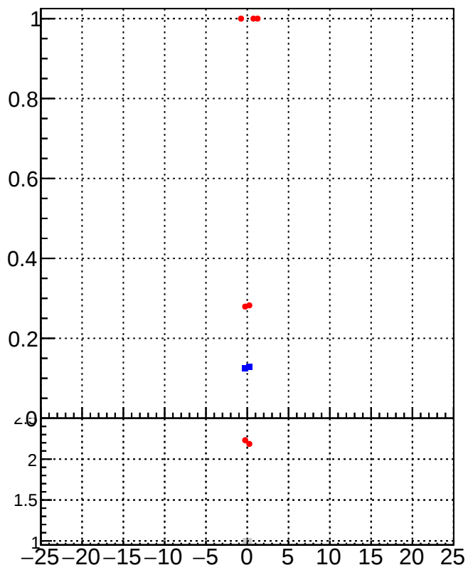
DQM_TT_mkFit_lowpT DQM_TT_mkFit_BDT_lowpT
