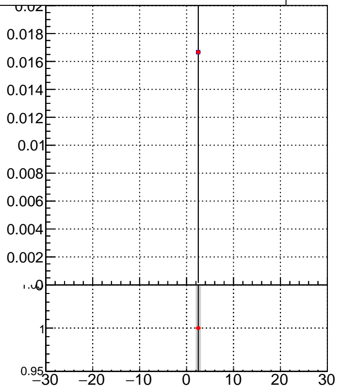
Legend: ■ DQM_TT_mkFit_lowpT ● DQM_TT_mkFit_BDT_lowpT
