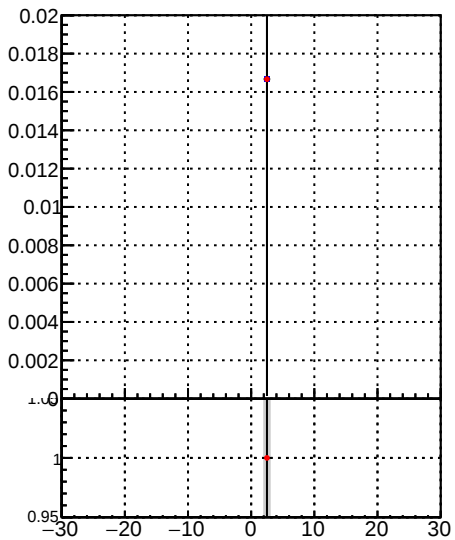
Fake rate vs d Legend: - DQM_TT_mkFit_lowpT (blue line with dots) - DQM_TT_mkFit_BDT_lowpT (red line with dots)
