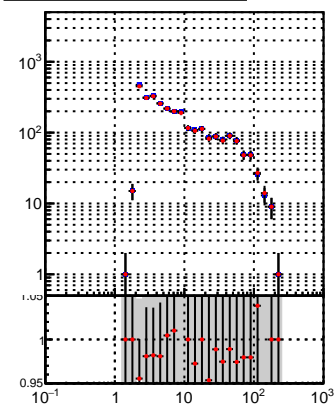
DQM_TT_mkFit_lowpT DQM_TT_mkFit_BDT_lowpT
