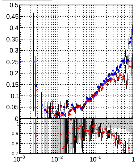
Legend: DQM_TT_mkFit_lowpT (blue squares), DQM_TT_mkFit_BDT_lowpT (red circles)
