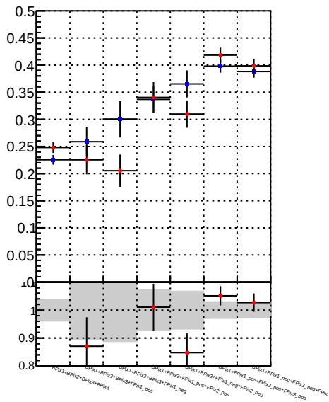
Fake rate vs. —●— DQM TT mkFit_lowpT —●— DQM TT mkFit_BDT_lowpT
