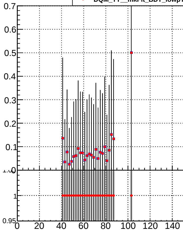
—■ DQM_TT_mkFit_lowpT —● DQM_TT_mkFit_BDT_lowpT
