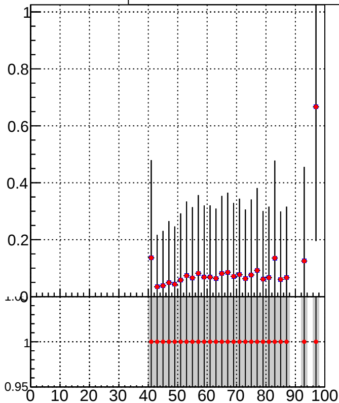
■ DQM_TT_mkFit_lowpT ● DQM_TT_mkFit_BDT_lowpT
