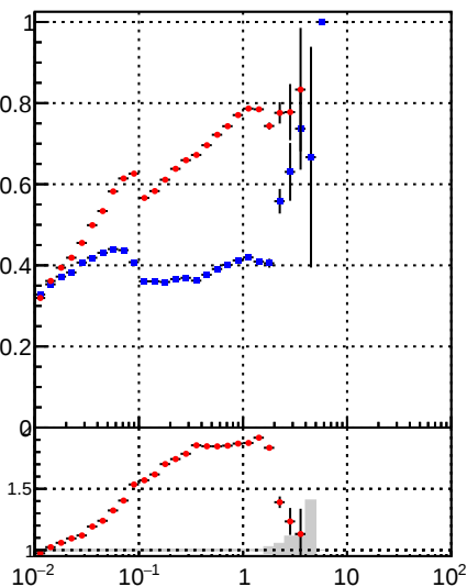
■ DQM_TT_mkFit_lowpT ● DQM_TT_mkFit_BDT_lowpT
