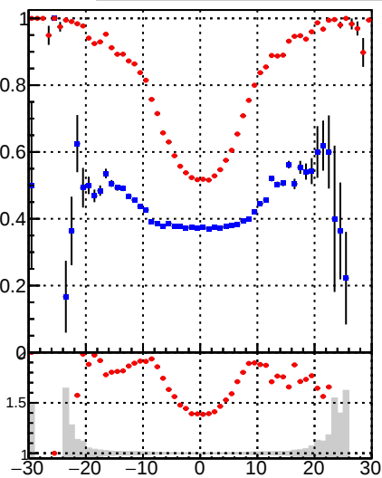
■ DQM_TT_mkFit_lowpT ● DQM_TT_mkFit_BDT_lowpT
