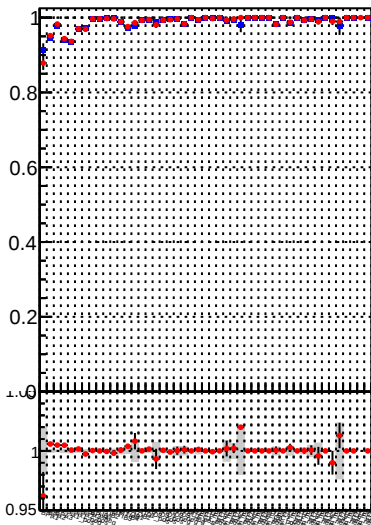
Fake rate vs. —●— DQM_TT_mkFit_lowpT —●— DQM_TT_mkFit_BDT_lowpT
