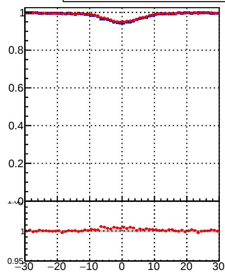
—•— DQM_TT_mkFit_lowpT —+— DQM_TT_mkFit_BDT_lowpT
