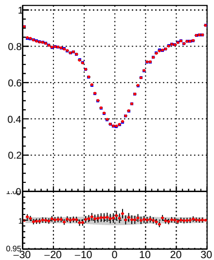
Fake rate vs d —●— DQM\_TT\_mkFit\_lowpT —●— DQM\_TT\_mkFit\_BDT\_lowpT
