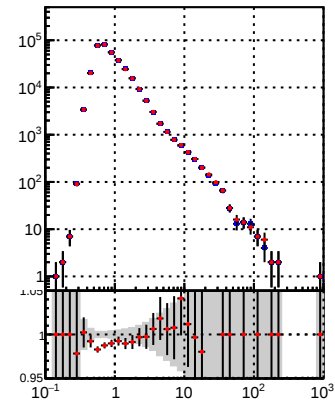
—•— DQM_TT_mkFit_lowpT —•— DQM_TT_mkFit_BDT_lowpT
