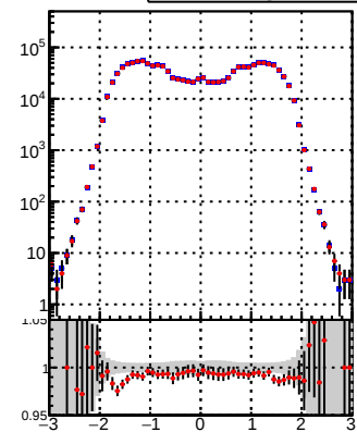
—•— DQM_TT_mkFit_lowpT —•— DQM_TT_mkFit_BDT_lowpT
