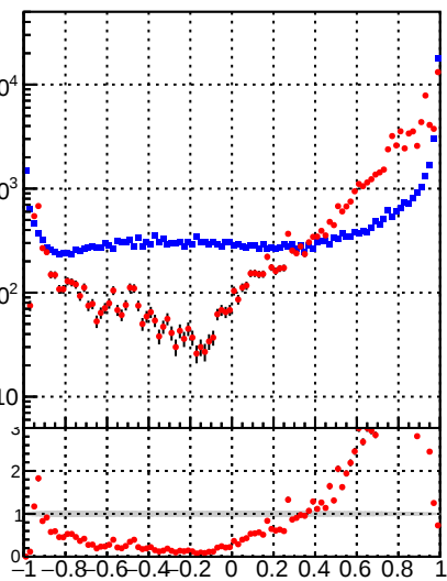
N of associated tracks (recoToSim) vs MVA1
