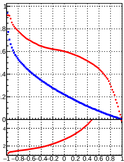
Fake rate vs. MVA1
