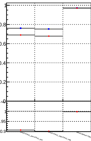
Fake rate vs. —●— DQM TT mkFit_lowpT —●— DQM TT mkFit_BDT_lowpT
