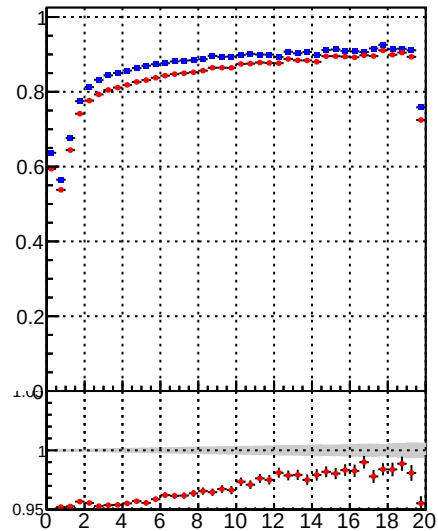
Fake rate vs. TT_mkFit_lowT TT_mkFit_BDT_lowT
