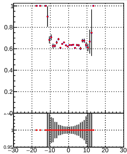
■ DQM_TT_mkFit_lowpT ● DQM_TT_mkFit_BDT_lowpT
