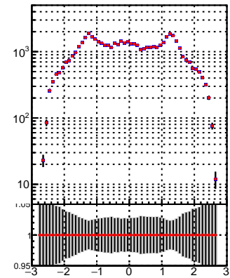
N of reco track vs \eta DQM_TT_mkFit_lowpT N of reco track vs \eta DQM_TT_mkFit_BDT_lowpT
