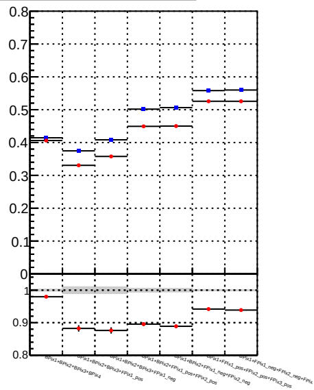
Fake rate vs. \chi^2
