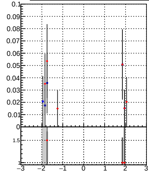
— DQM_TT_mkFit_lowpT — DQM_TT_mkFit_BDT_lowpT
