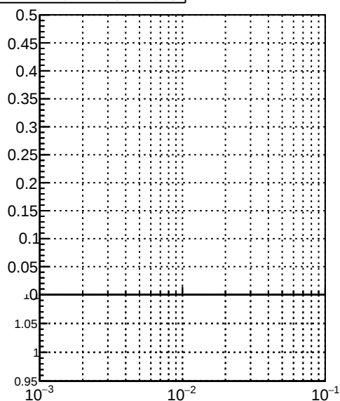
Efficiency vs \Delta R(\text{track, jet})
