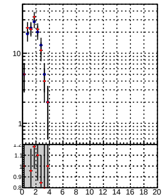
N of reco track vs. s DQM TT mkFit_lowT DQM TT mkFit_BDT_lowT
