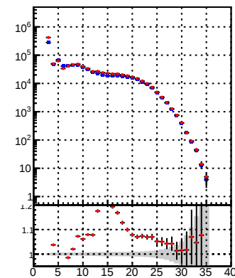
—•— DQM_TT_mkFit_lowpT —•— DQM_TT_mkFit_BDT_lowpT
