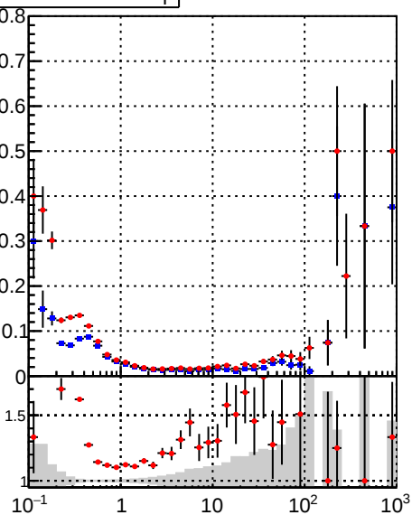
fake+duplicates vs p_T
