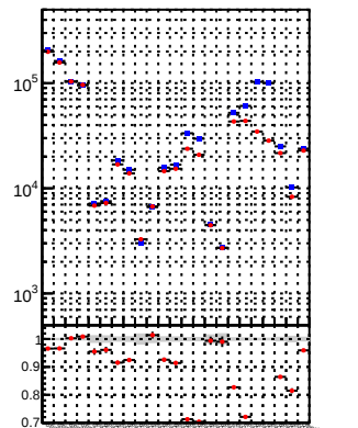
N of reco track vs. \chi^2
