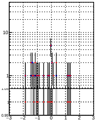
N of reco track vs \eta DQM TT mkFit lowpT DQM TT mkFit BDT lowpT
