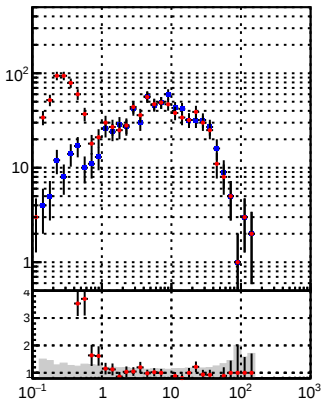
—•— DQM_TT_mkFit_lowpT —•— DQM_TT_mkFit_BDT_lowpT
