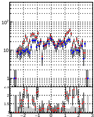
—•— DQM_TT_mkFit_lowpT —•— DQM_TT_mkFit_BDT_lowpT
