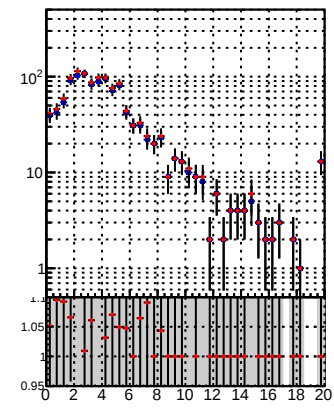
N of reco track vs. \chi^2 DQM TT mkFit_lowpT DQM TT mkFit_BDT_lowpT
