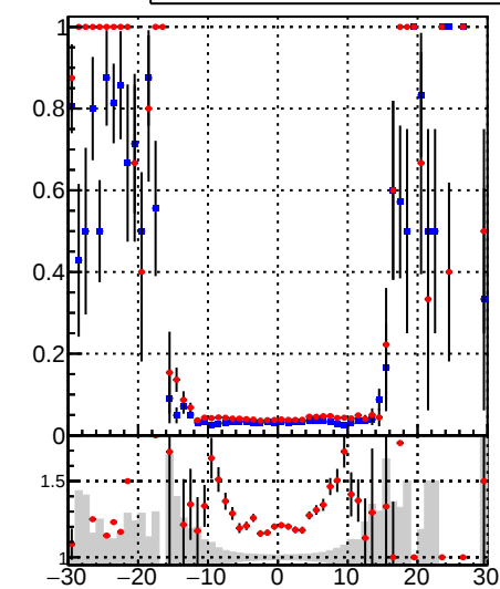
—■— DQM_TT_mkFit_lowpT —+— DQM_TT_mkFit_BDT_lowpT
