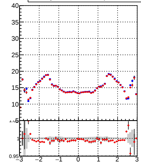
mean hit — DQM_TT_mkFit_lowpT — DQM_TT_mkFit_BDT_lowpT
