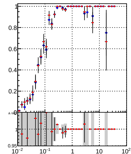
Legend: DQM_TT_mkFit_lowpT (blue squares) DQM_TT_mkFit_BDT_lowpT (red circles) Fake rate vs vertpos
