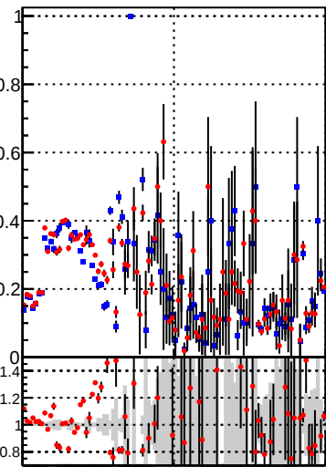
Fake rate vs. —●— DQM_TT_mkFit_lowpT —●— DQM_TT_mkFit_BDT_lowpT
