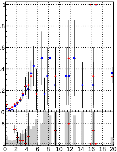
Fake rate vs. —•— DQM_TT_mkFit_lowpT —•— DQM_TT_mkFit_BDT_lowpT
