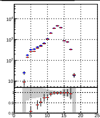
—•— DQM_TT_mkFit_lowpT —•— DQM_TT_mkFit_BDT_lowpT
