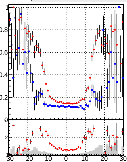
■ DQM_TT_mkFit_lowpT ■ DQM_TT_mkFit_BDT_lowpT
