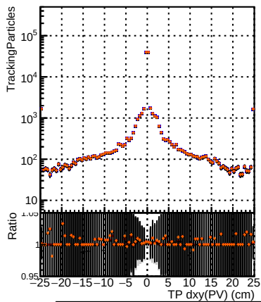
Legend for N of simulated tracks vs dxy(PV): DQM_mkFit_TToriginal (blue line) DQM_mkFit_TTNEWnoMS-genMatch-chi200 (red line) DQM_mkFit_TToriginal-106 (black line) DQM_mkFit_TTNEWMS-genMatch-chi200 (orange line)
