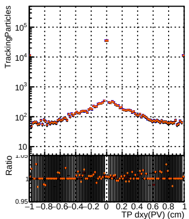
— DQM_mkFit_TToriginal — DQM_mkFit_TTNEWnoMS-genMatch-chi200 — DQM_mkFit_TToriginal-106 — DQM_mkFit_TTNEWMS-genMatch-chi200
