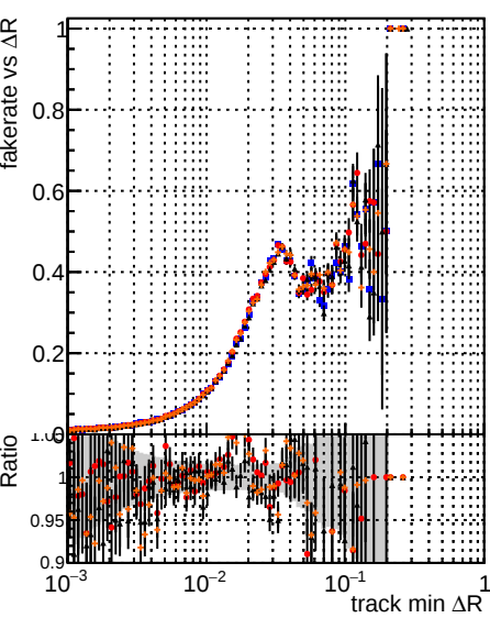
Fake rate vs \Delta R (track, jet) DOM mktFit TOriginal MS-genMatch-chi200 DOM mktFit TOriginal MS-genMatch-chi200 DOM mktFit TOriginal MS-genMatch-chi200
