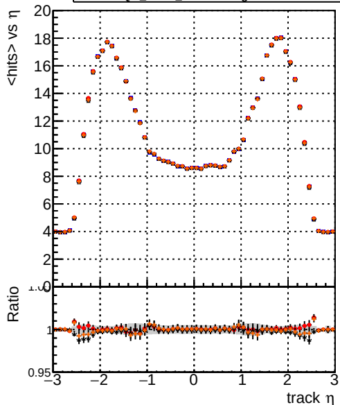
DQM_mkFit_TToriginal DQM_mkFit_TTNEWnoMS-genMatch-chi200 DQM_mkFit_TToriginal-106 DQM_mkFit_TTNEWMS-genMatch-chi200 mean hit
