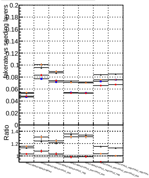
Fake rate vs. BQM mkFit + TtoWMS-genMatch-chi200 BQM mkFit + TtoWMS-genMatch-chi200 BQM mkFit + TtoWMS-genMatch-chi200
