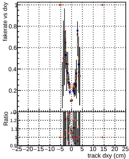
DOM mkt Fit T Original MS-genMatch-chi200 DOM mkt Fit T Original MS-genMatch-chi200
