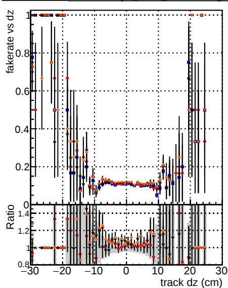
DOM mkt Fit T Original MS-genMatch-chi200 DOM mkt Fit T Original MS-genMatch-chi200
