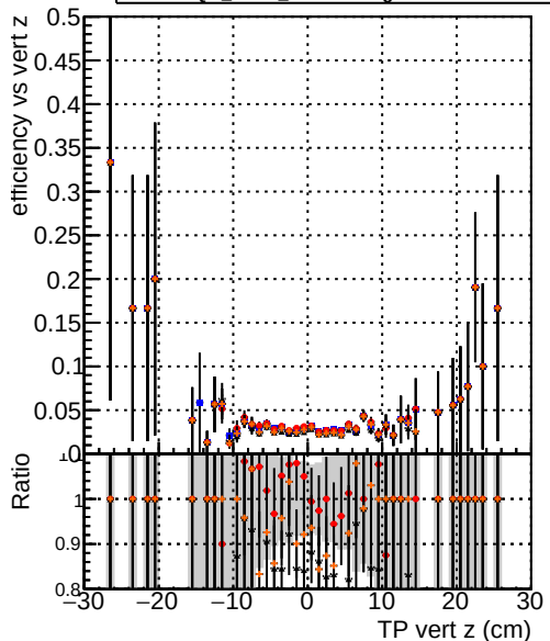
Efficiency vs. TP vert z (cm) —•— DQM_mkFit_TToriginal —•— DQM_mkFit_TTNEwMS-genMatch-chi200 —•— DQM_mkFit_TToriginal-106 —•— DQM_mkFit_TTNEwMS-genMatch-chi200
