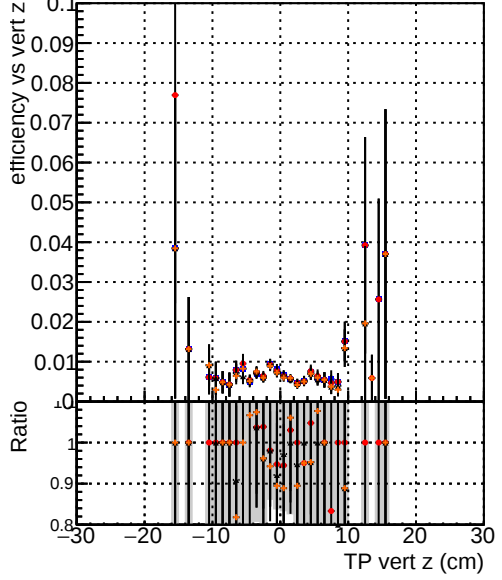
Efficiency vs. TP vert z (cm) DOM_mkFit_TToriginal DOM_mkFit_TTNEWnoMS-genMatch-chi200 DOM_mkFit_TToriginal-106 DOM_mkFit_TTNEWMS-genMatch-chi200
