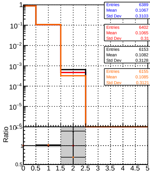
mean hit DQM_mkFit_TToriginal DQM_mkFit_TTNEWnoMS-genMatch-chi200 DQM_mkFit_TToriginal-106 DQM_mkFit_TTNEWMS-genMatch-chi200
