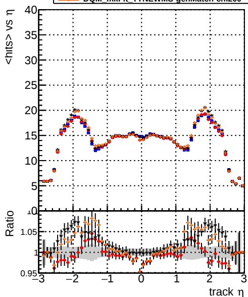
Legend: DQM_mkFit_TToriginal (blue), DQM_mkFit_TTNEWnoMS-genMatch-chi200 (red), DQM_mkFit_TToriginal-106 (black), DQM_mkFit_TTNEWMS-genMatch-chi200 (orange) mean hit
