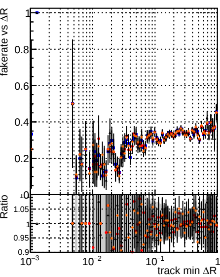
Fake rate vs \Delta R(\text{track, jet}) DQM mktFit TToriginal MS-genMatch-chi200 DQM mktFit TToriginal MS-genMatch-chi200 DQM mktFit TToriginal MS-genMatch-chi200
