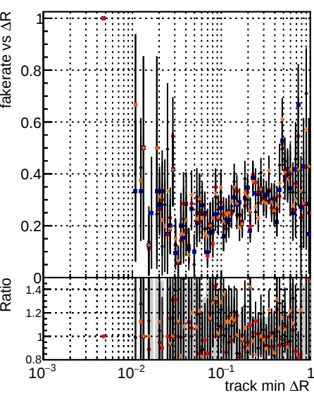
Fake rate vs \Delta R(\text{track, jet}) for MS-genMatch-chi200, Wino-100, and MS-genMatch-chi200. Legend: DOM (black), mktFit (blue), T-Original (red), and T-NEWMS-genMatch-chi200 (orange).
